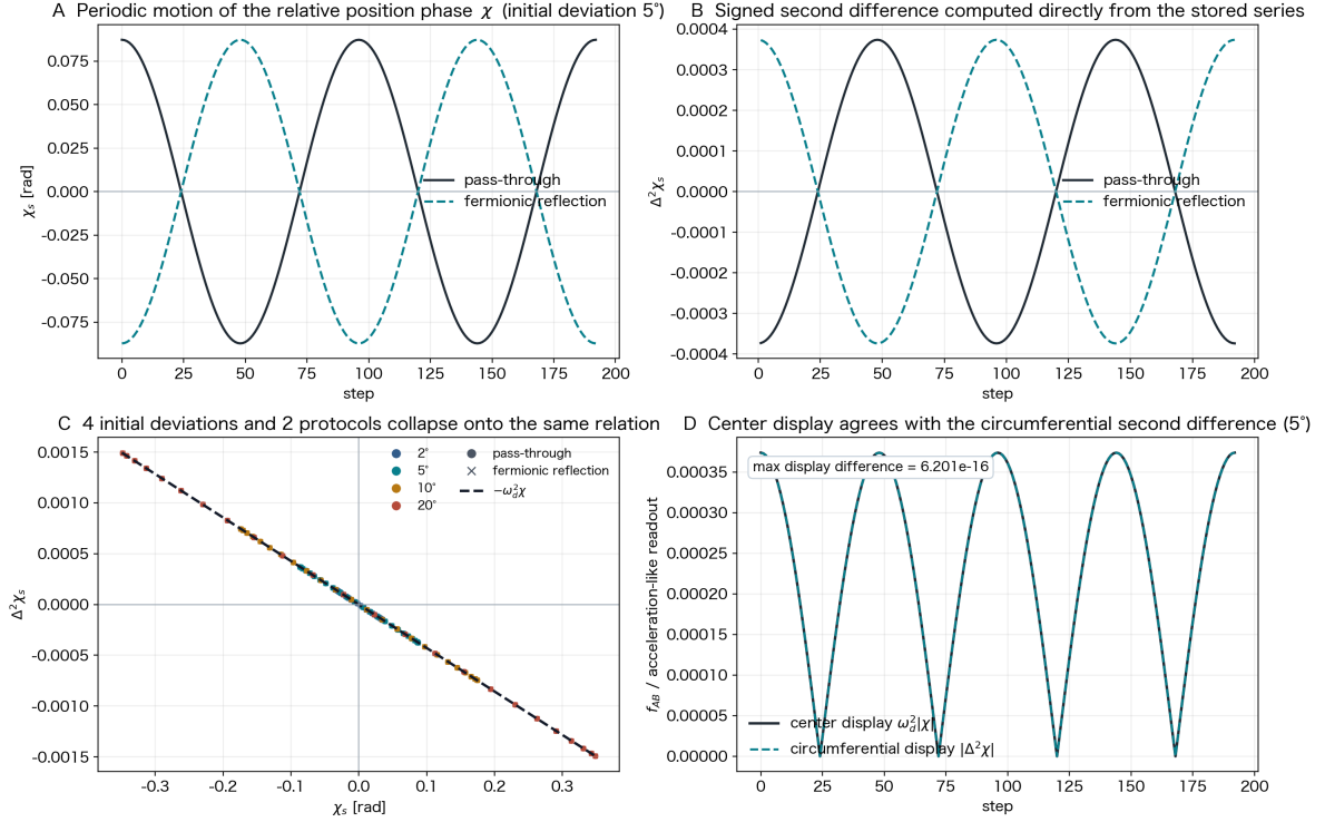
Published AB acceleration experiment: nonzero second difference and the harmonic acceleration relation
