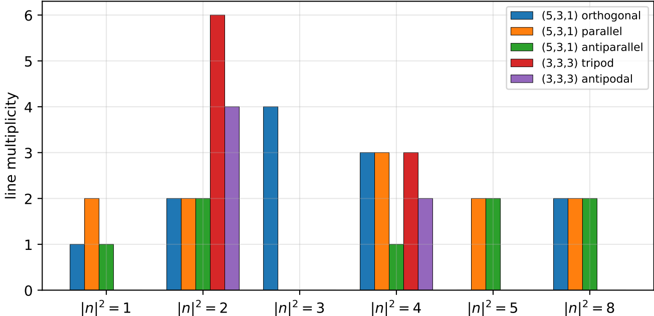
Power-spectrum line tables separate all five relation classes (unit-record readable)
