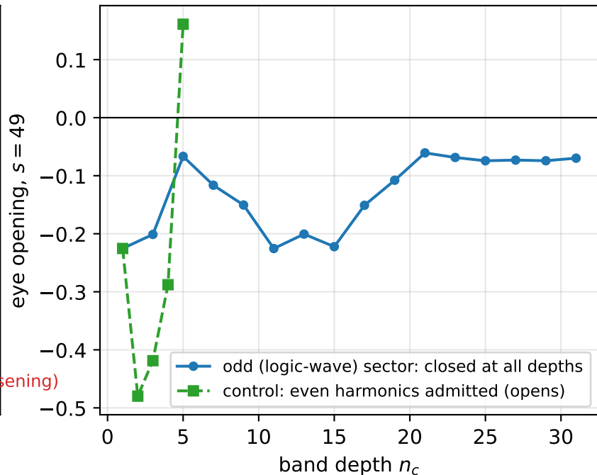
(a) Three bands: certified \{1, 3, 5\} / critical 7–21 / forbidden \geq 25 (b) Closure is specific to the odd sector ( s = 49 )
