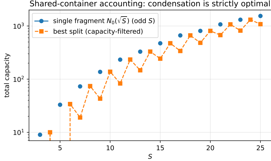
Figure 1: Figure 1. Condensation optimality under the shared container
