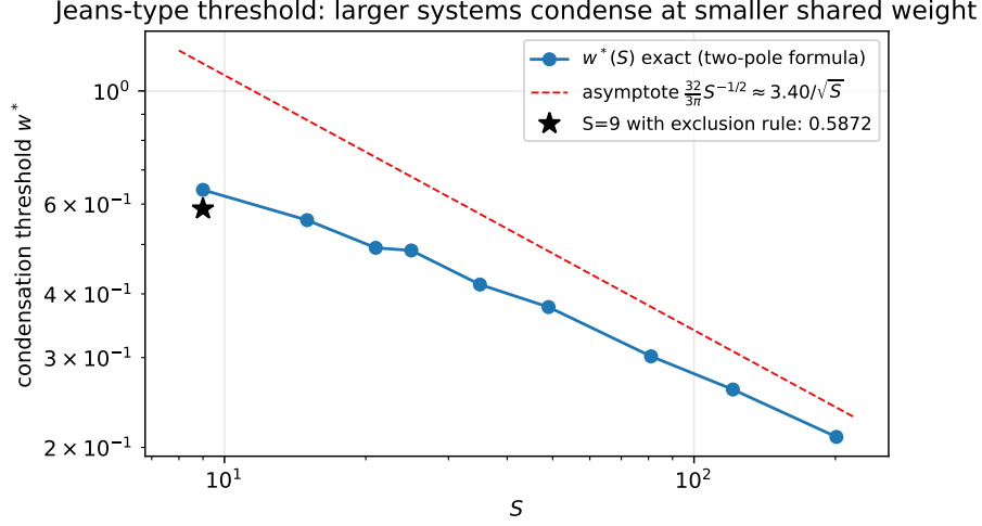
Figure 2: Figure 2. Jeans-type condensation threshold
