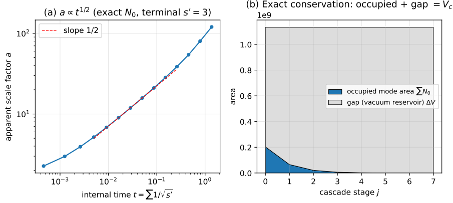
Figure 3: Figure 3. Internal expansion law and the vacuum reservoir
