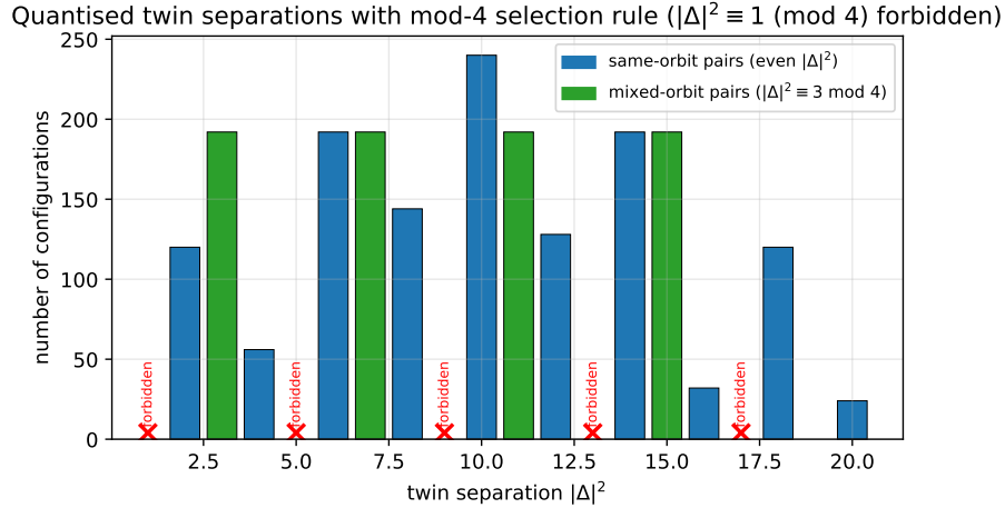
Figure 3: Figure 3. Quantised twin separations with the mod-4 selection rule
