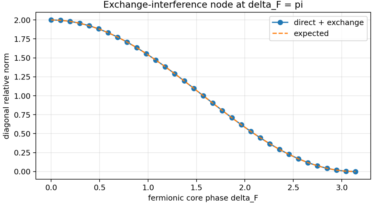
Figure 2: Exchange-interference phase sweep
