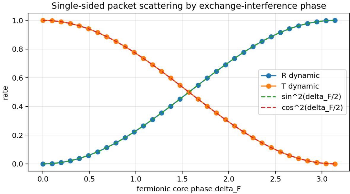
Figure 1: One-sided scattering
