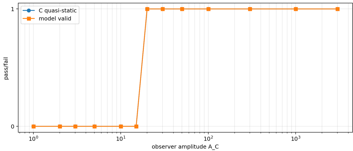
Figure 6: Observer validity
