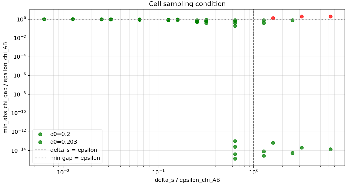
Figure 7: Sampling condition
