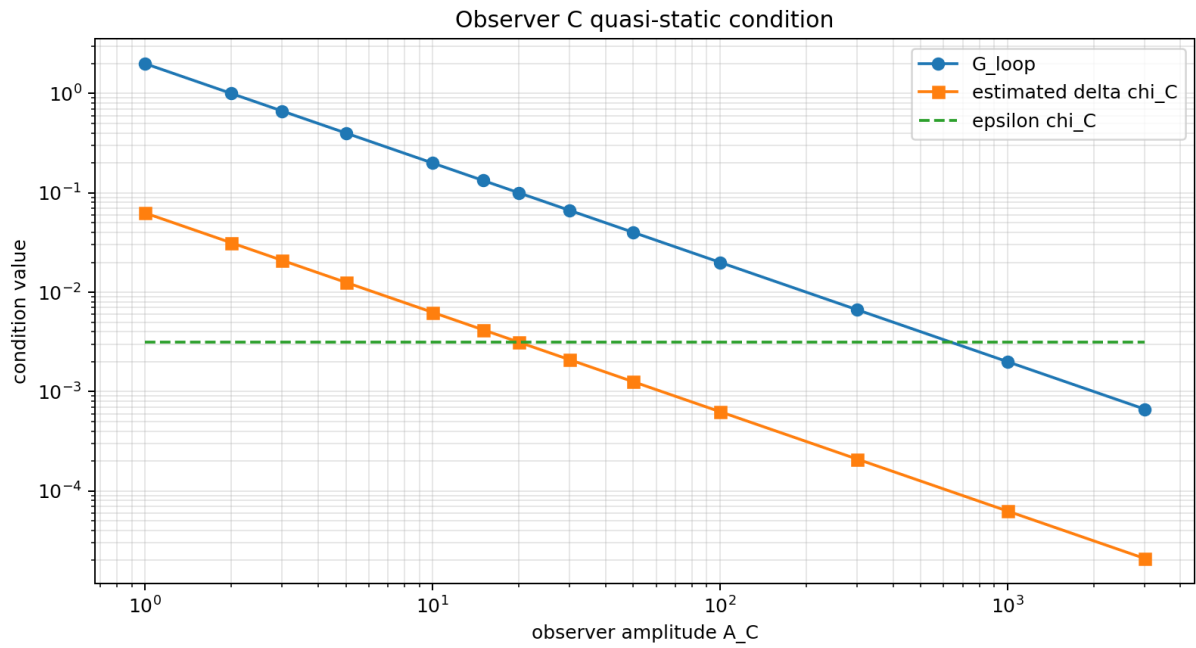
Figure 5: Observer conditions
