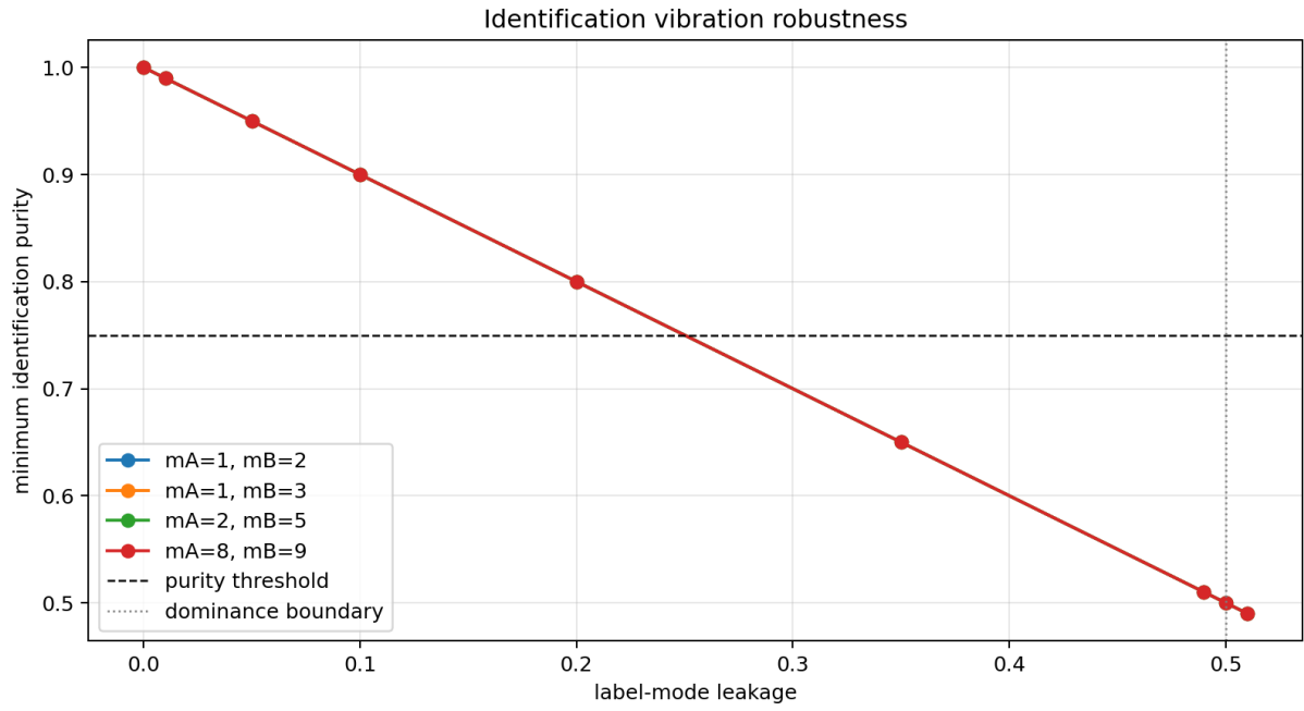
Figure 3: Identification purity
