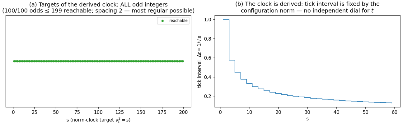
- Figure 3 (paper13_fig3_derived_time.png): (a) clock targets = all odds (100/100 below 199, spacing 2). (b) tick \Delta t = 1/\sqrt{s} — no independent scale for t
