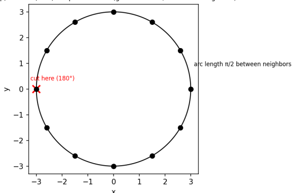
Fig.A The 1+1D map ( R=3 ): geodesic-length-preserving — spacing is invariant (reference, zero distortion)
