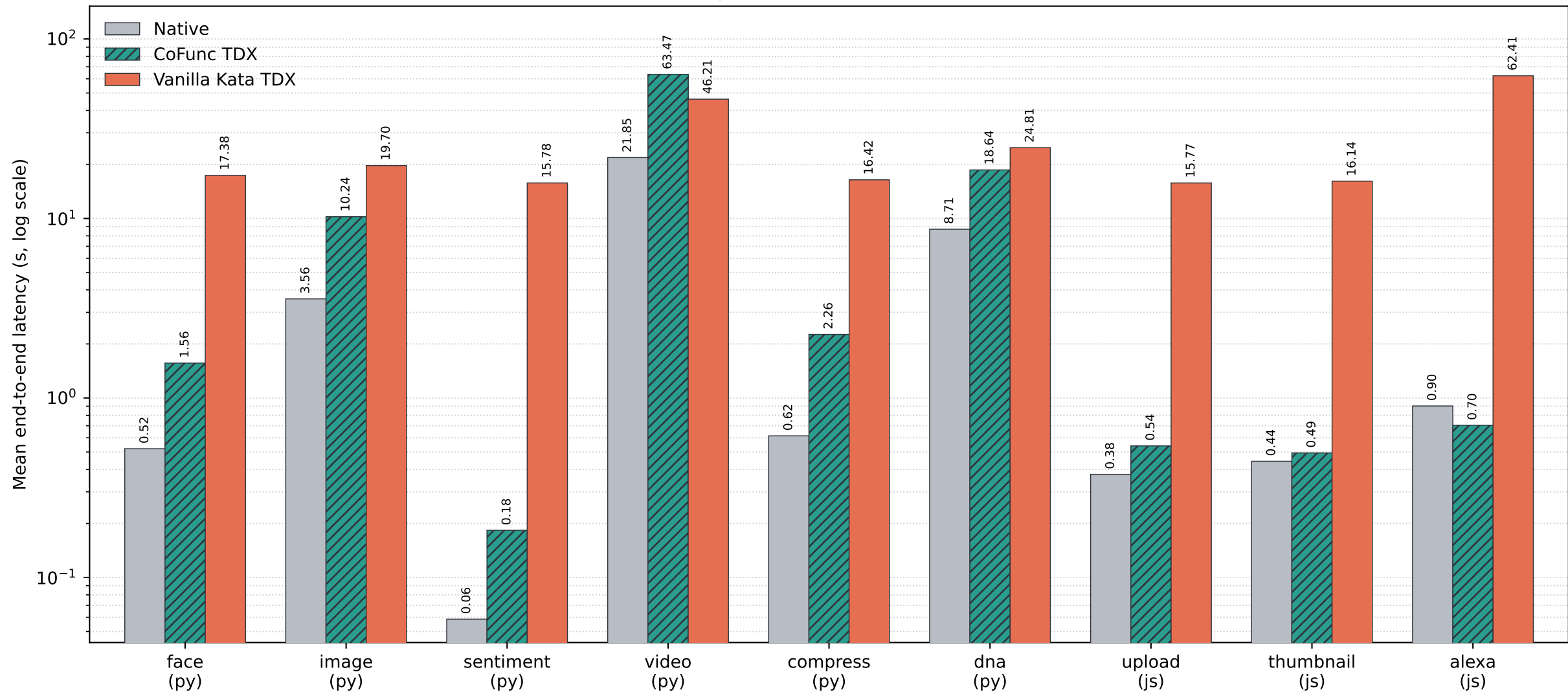
Measured TDX Fig. 11: Native vs CoFunc vs Vanilla Kata
