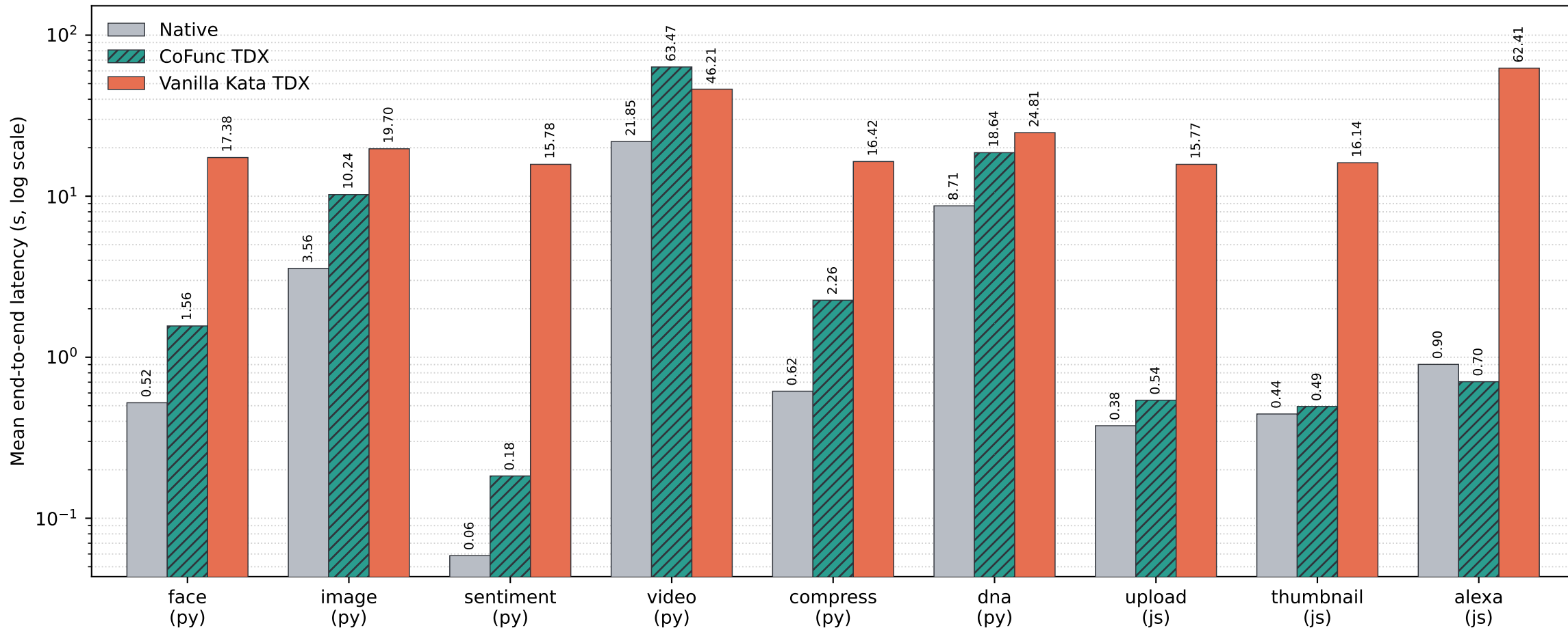
Measured TDX Fig. 11: Native vs CoFunc vs Vanilla Kata
