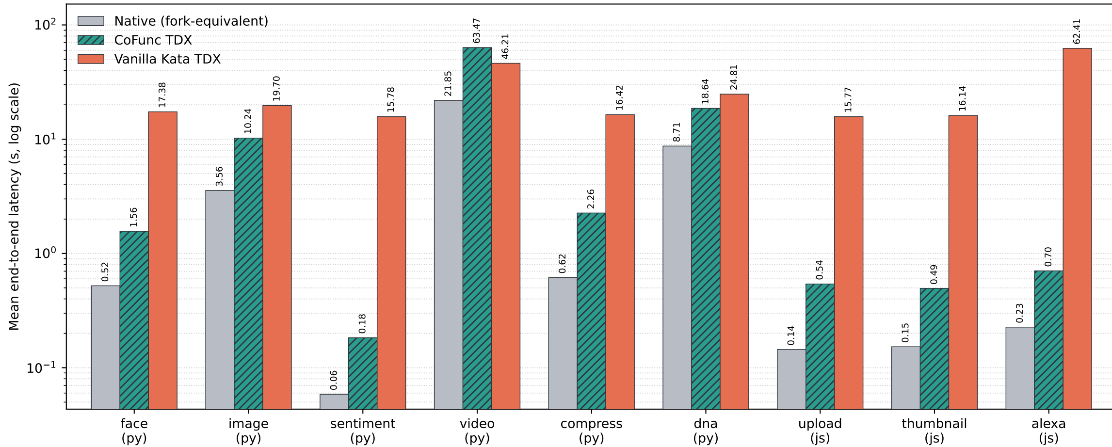
Paper-aligned measured TDX Fig. 11
