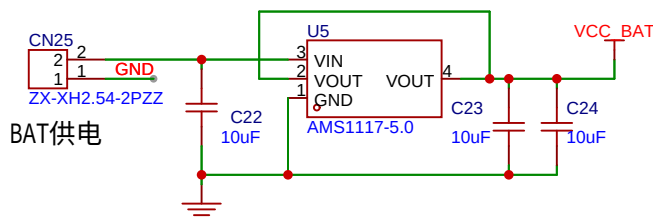
7.4V转5V
