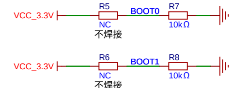
BOOT
