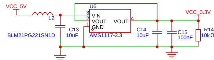
5V转3.3V
