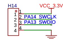
SWD Load
