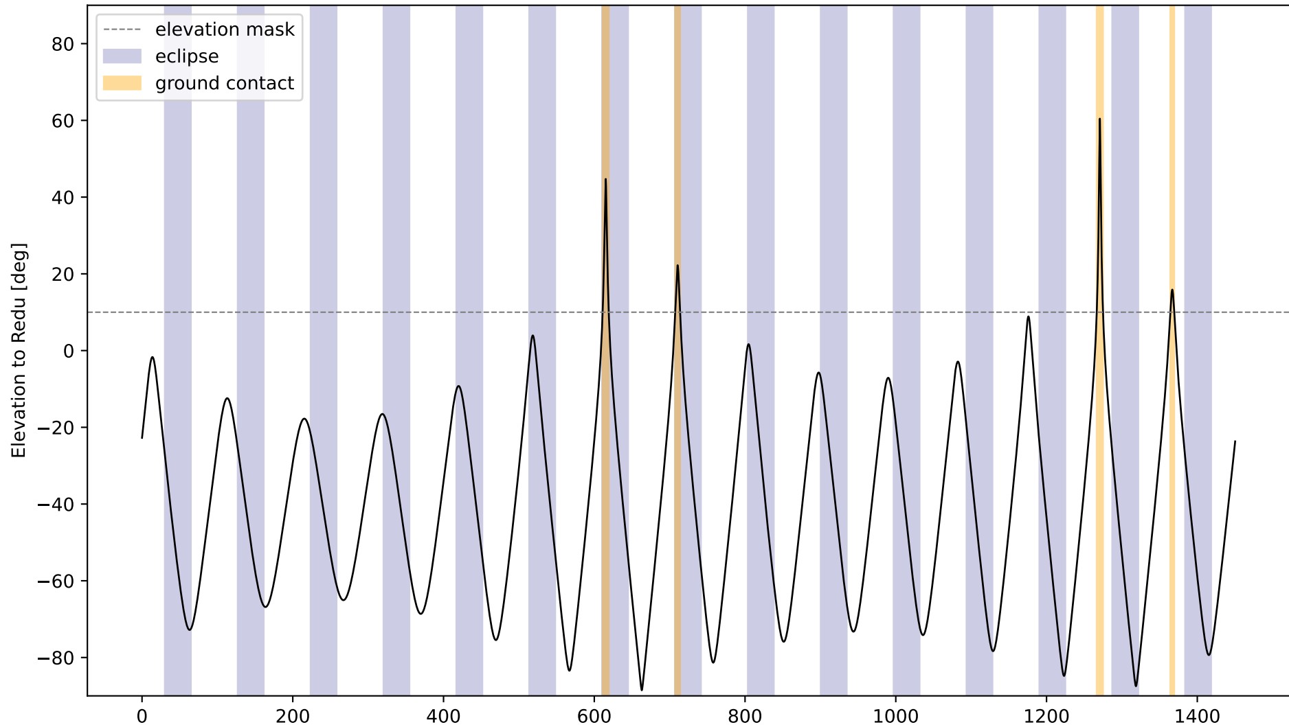
Orbit geometry over 15 orbit(s) (T = 96.69 min), 600 km SSO
