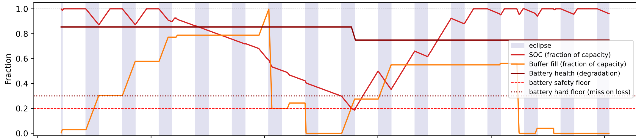
Episode trajectory (total reward=52, terminated=False)
