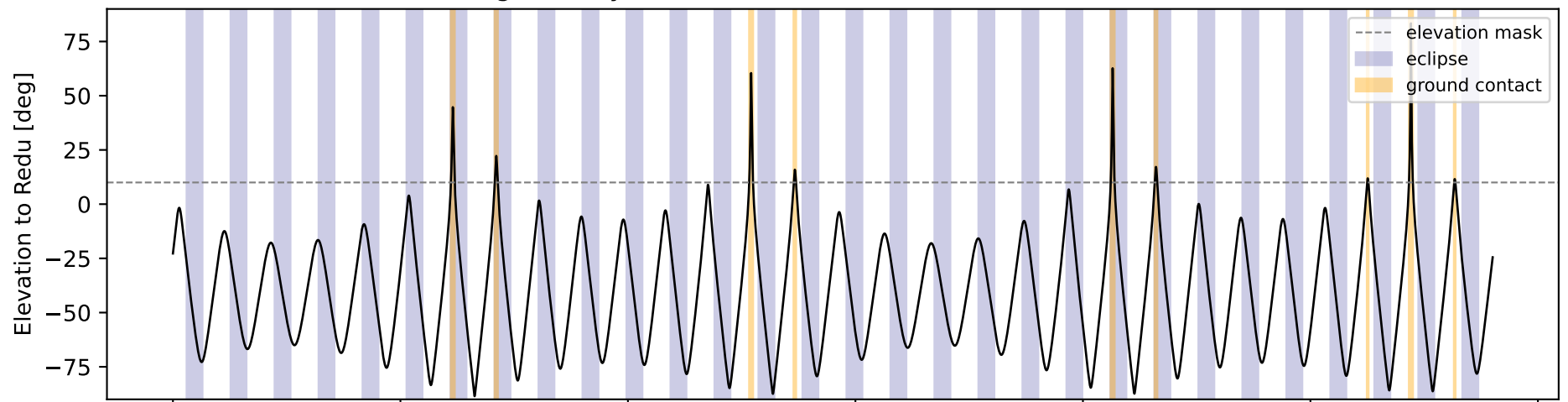
Orbit geometry over 30 orbit(s) (T = 96.69 min), 600 km SSO
