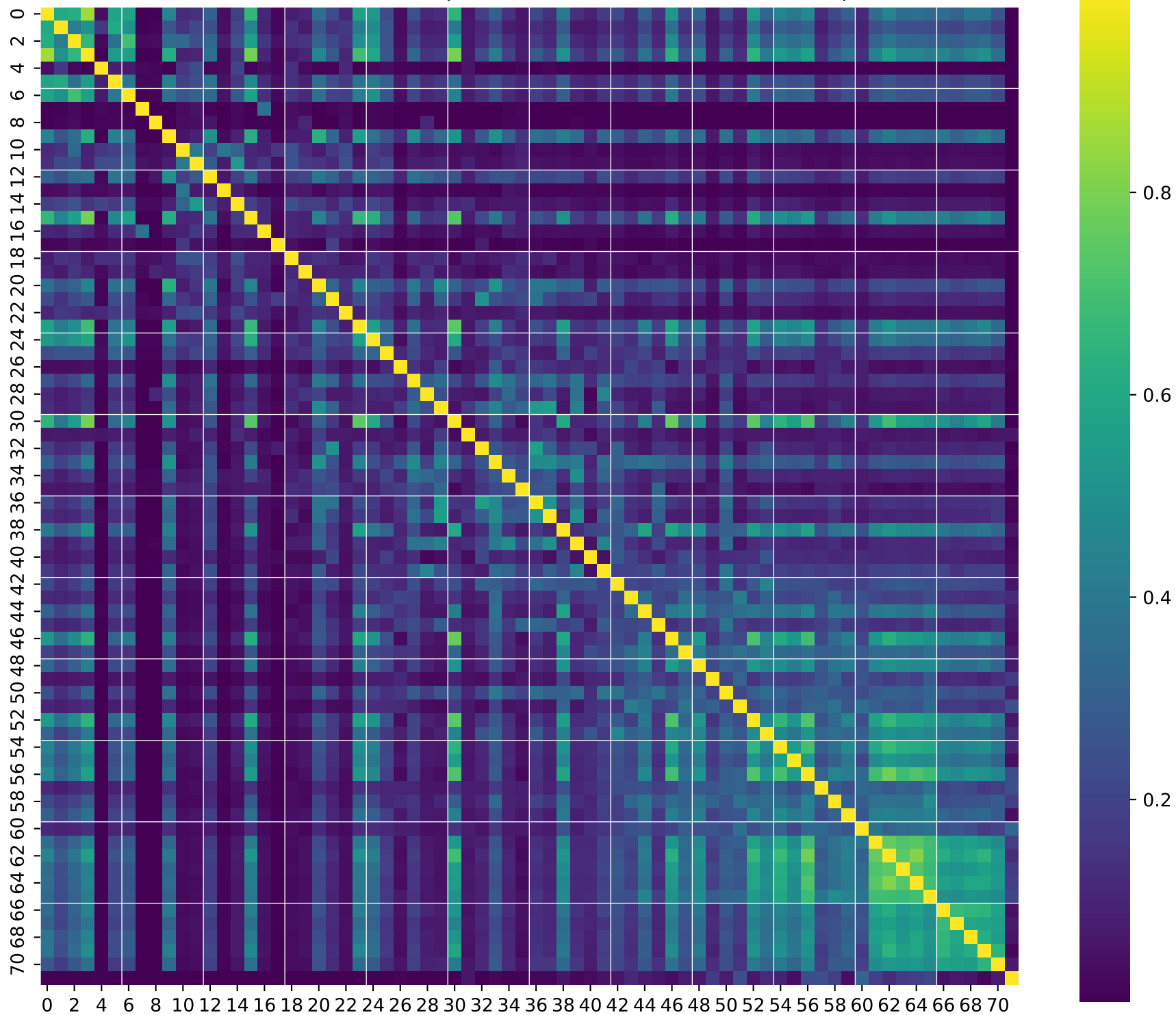
CKA: facebook/deit-small-patch16-224 on CIFAR100 (500 samples)
