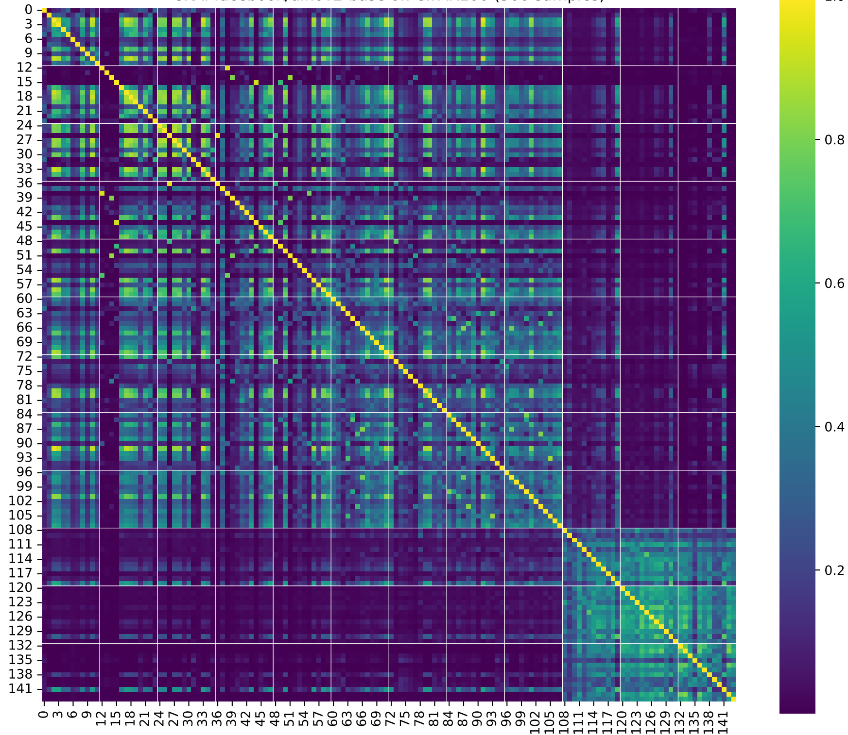
CKA: facebook/dinov2-base on CIFAR100 (500 samples)
