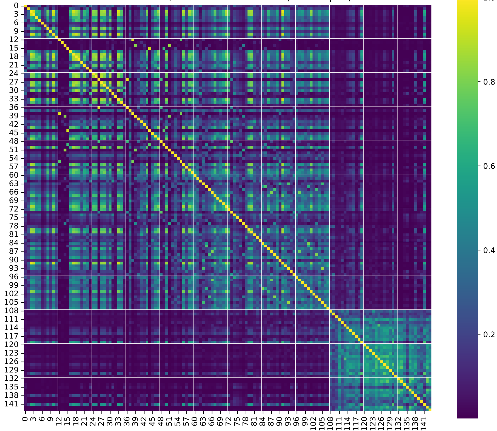
CKA: facebook/dinov2-base on CIFAR10 (500 samples)
