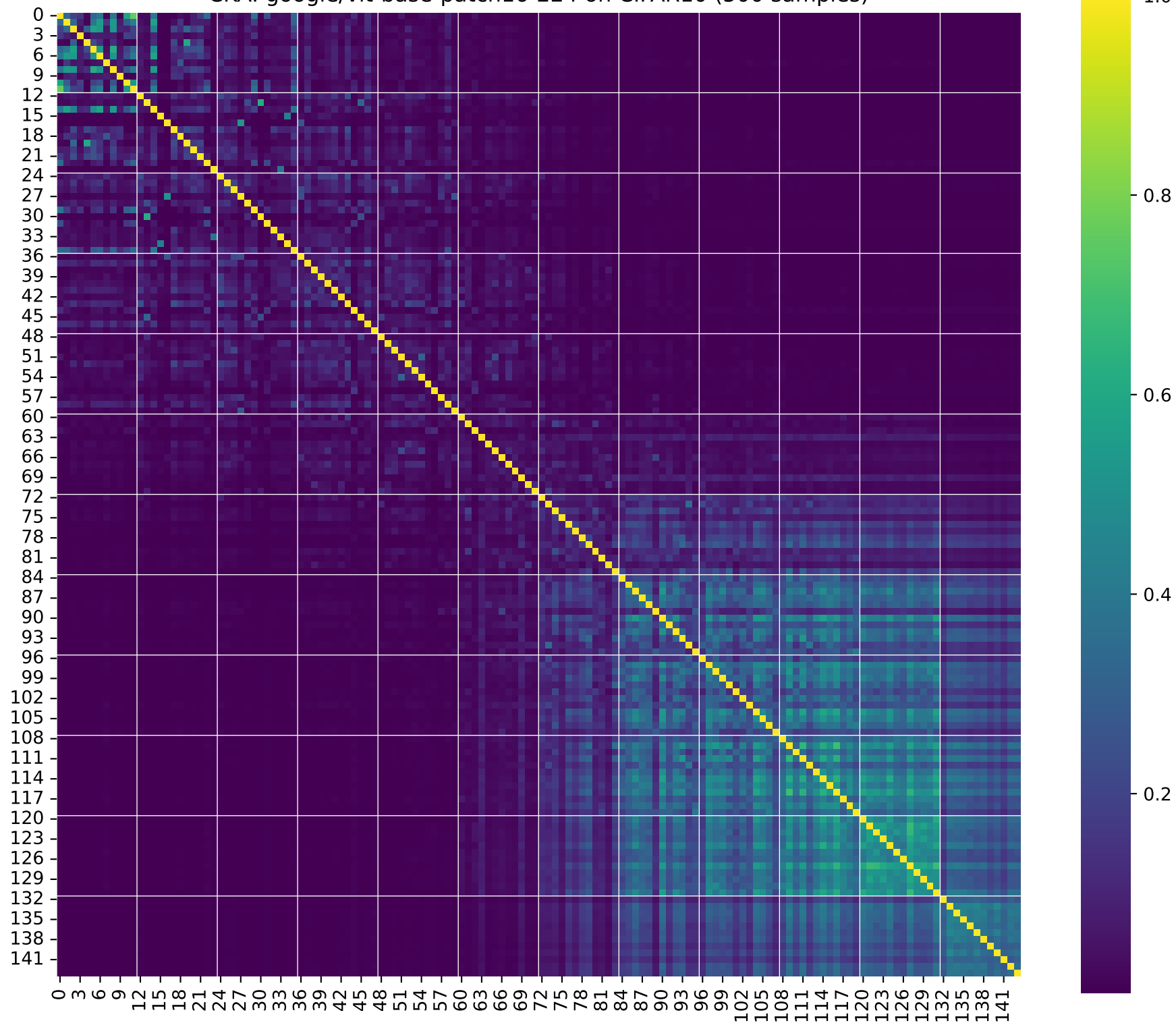
CKA: google/vit-base-patch16-224 on CIFAR10 (500 samples)
