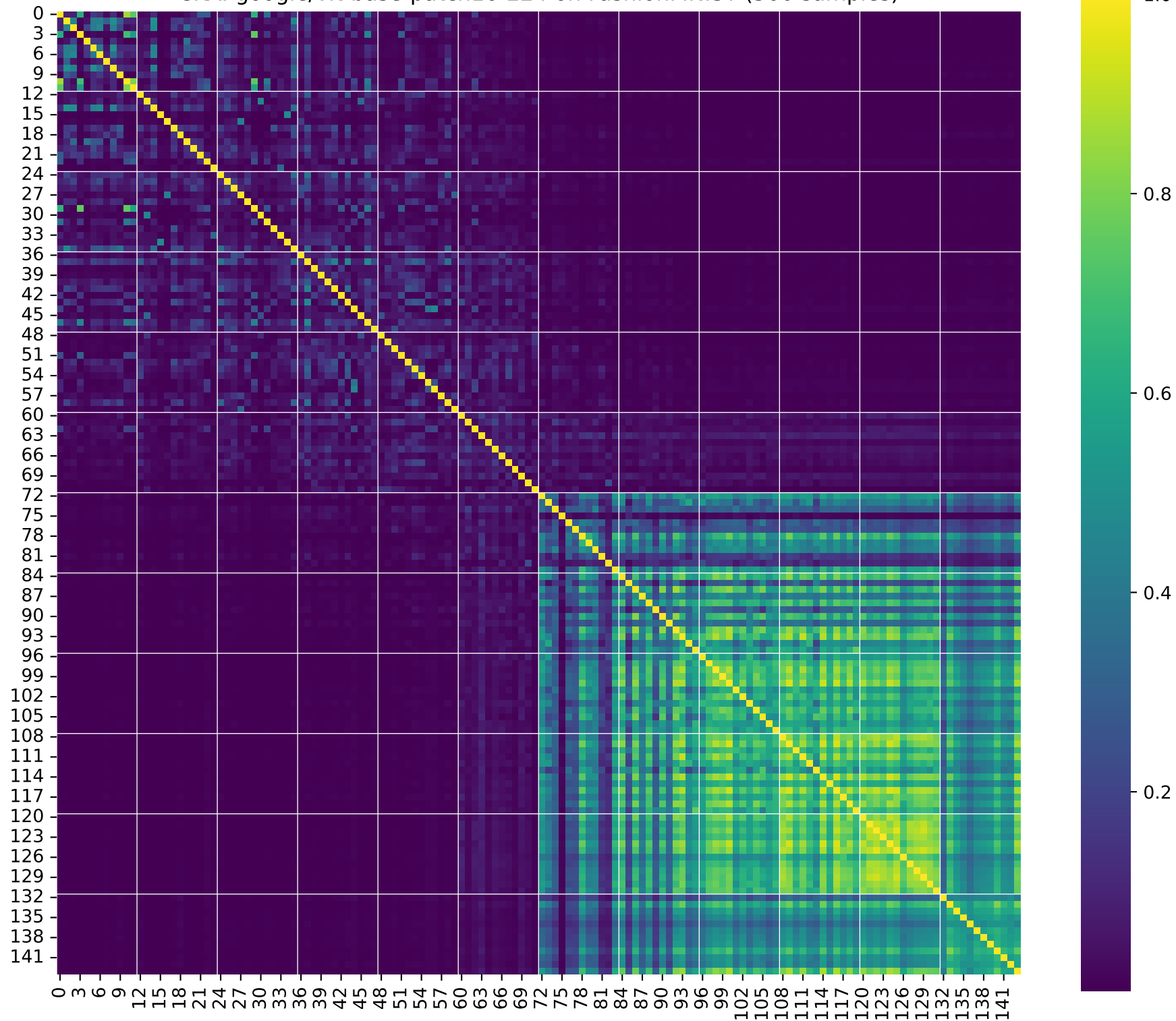
CKA: google/vit-base-patch16-224 on FashionMNIST (500 samples)
