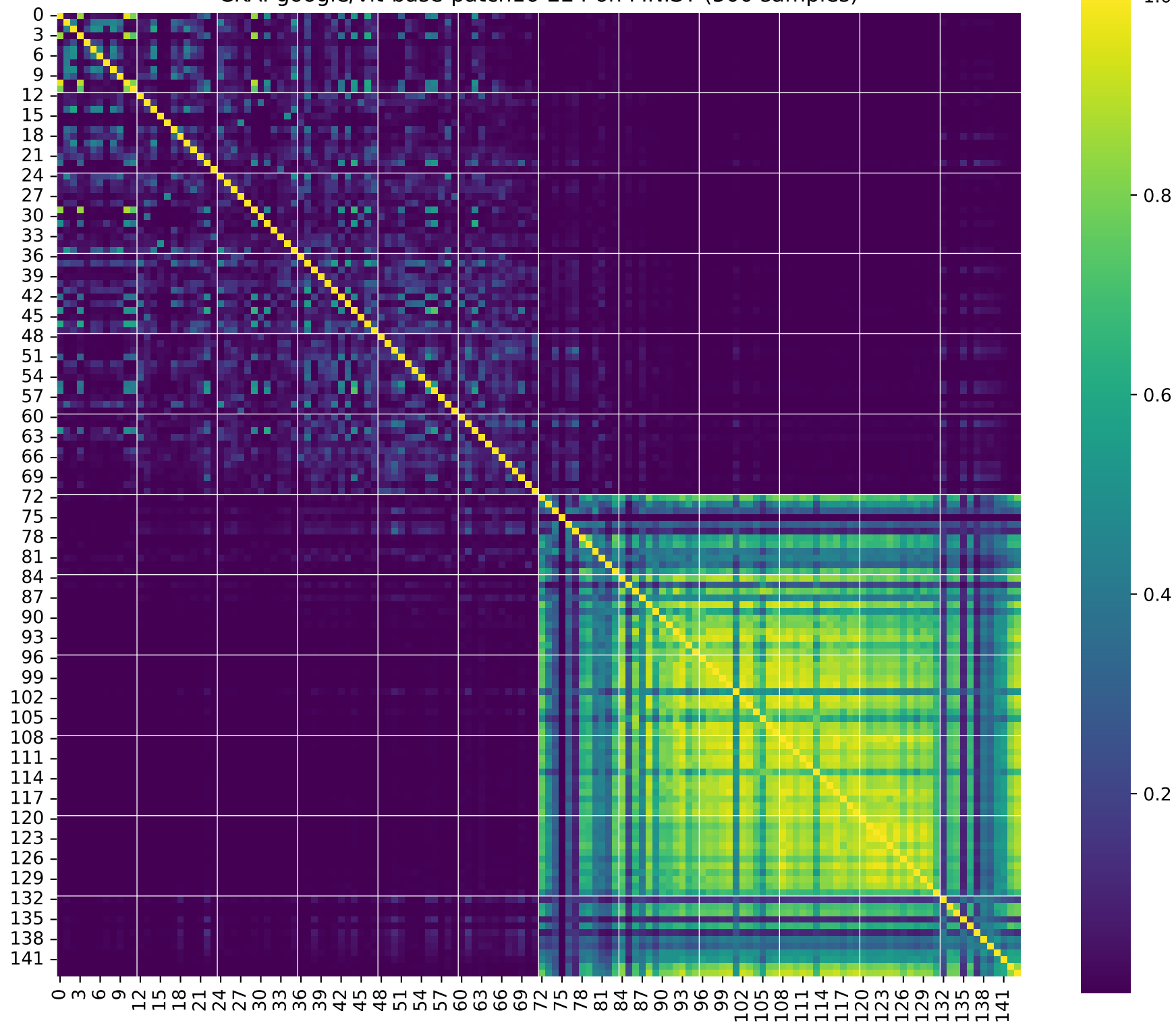
CKA: google/vit-base-patch16-224 on MNIST (500 samples)
