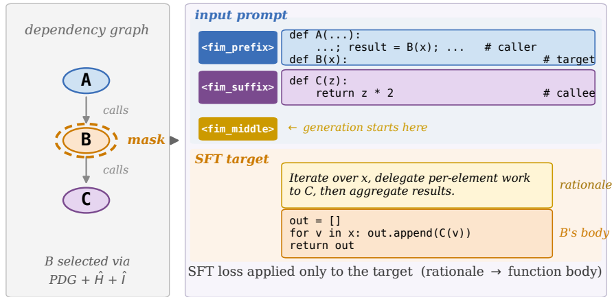
Function-level FIM mid-training (SFT)
