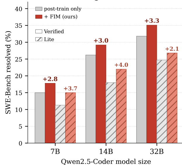
SWE-Bench gain across scales
