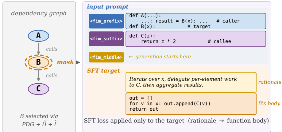
Function-level FIM mid-training (SFT)
