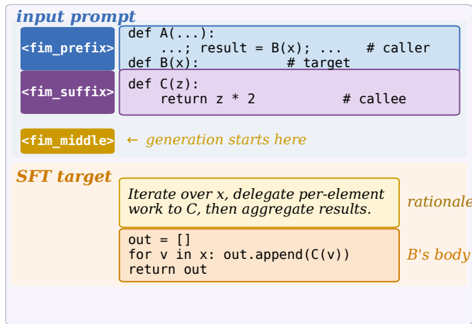
Function-level FIM mid-training (SFT)
