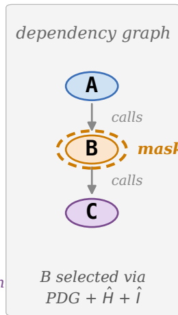
Function-level FIM mid-training (SFT)
