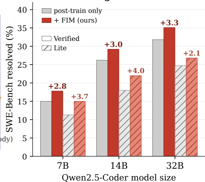
SWE-Bench gain across scales
