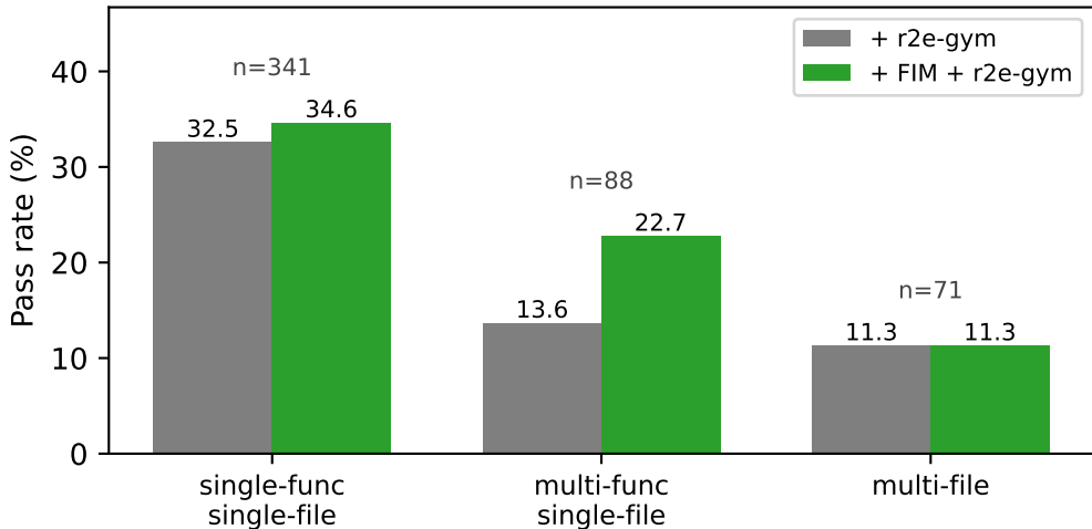
Pass rate by gold-patch shape (SWE-Bench-Verified)
