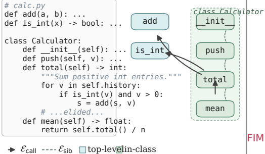
(a) Program dependency graph
