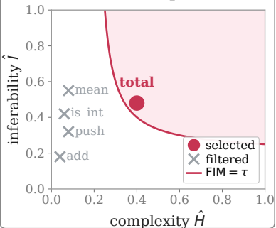
(c) Selection in \hat{H} - \hat{I} plane
