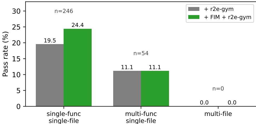
Pass rate by gold-patch shape (SWE-Bench-Lite)
