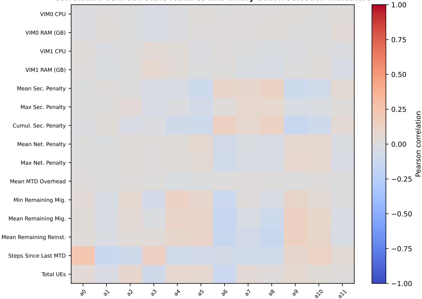
A2C - Feature <-> Action Selection (full log, 5,000 rows) Correlation between state features and binary action-selection indicators
