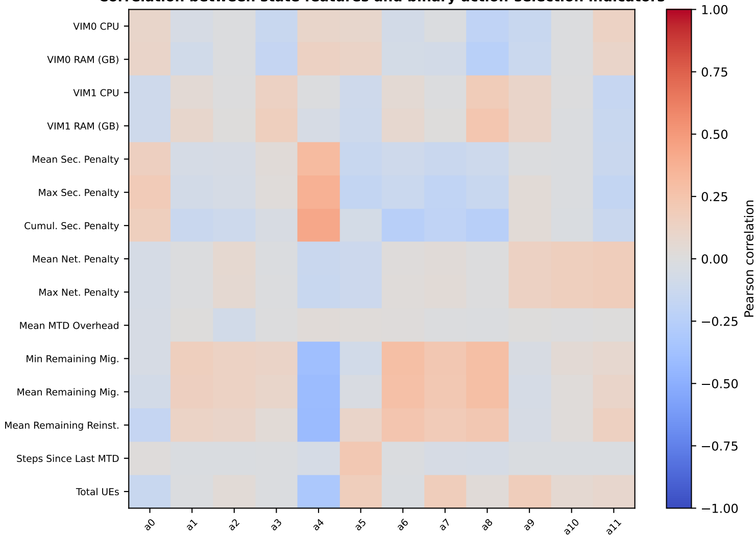
DQN - Feature <=> Action Selection (full log, 5,000 rows) Correlation between state features and binary action-selection indicators
