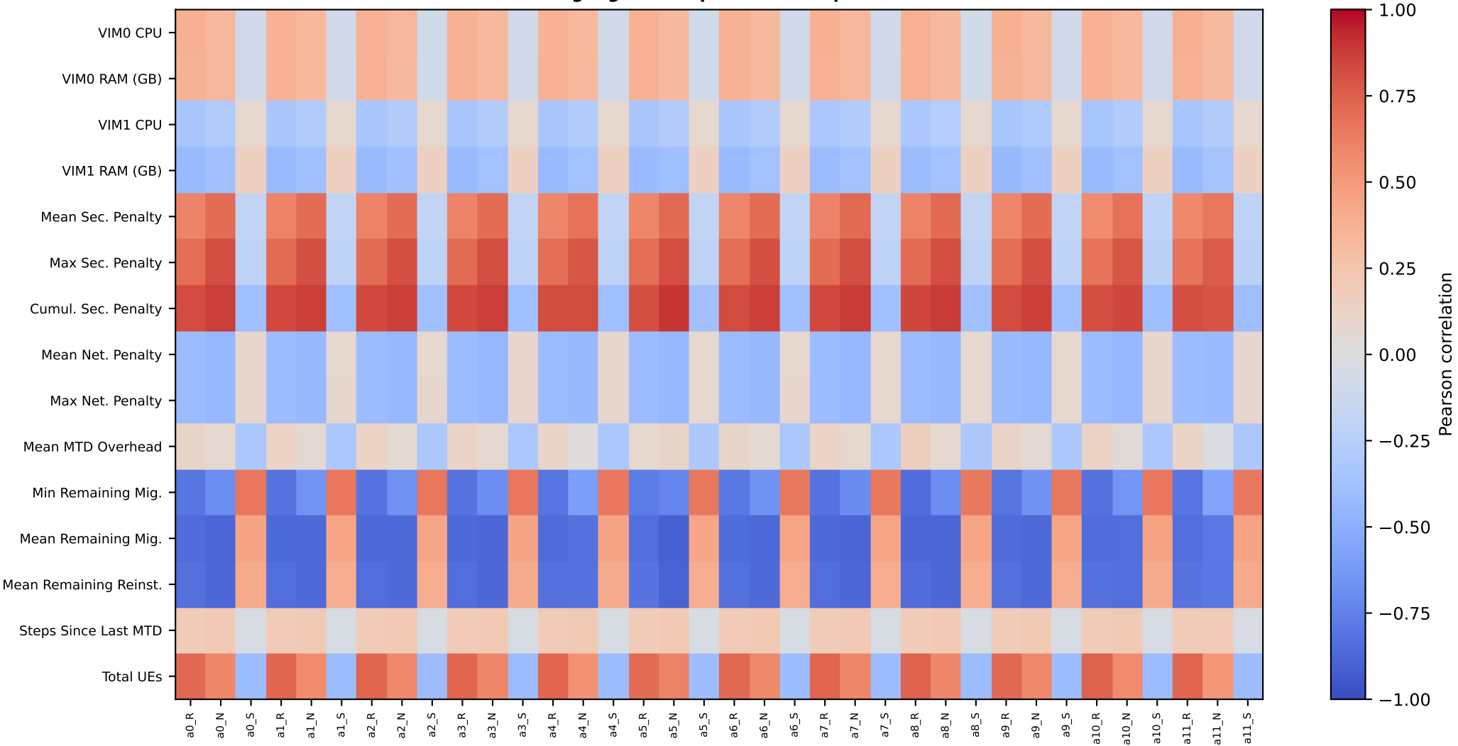
EUPG - Feature ↔ Q-value Correlation (full log, 5,000 rows) Highlighted step context: step 186
