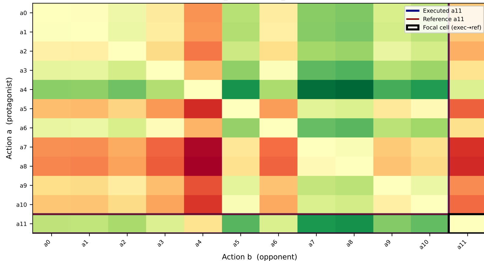
EUPG - Pairwise Q Advantage at Step 186 [Advantage] cell (a,b) = scalar_Q(a) – scalar_Q(b) >0: a is better
