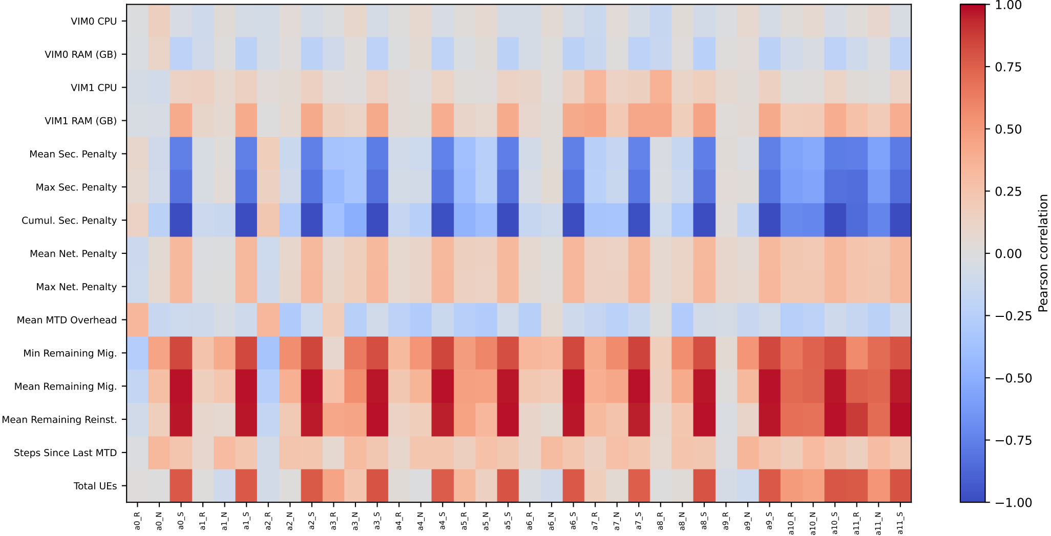
Envelope - Feature ↔ Q-value Correlation (full log, 5,000 rows) Highlighted step context: step 111
