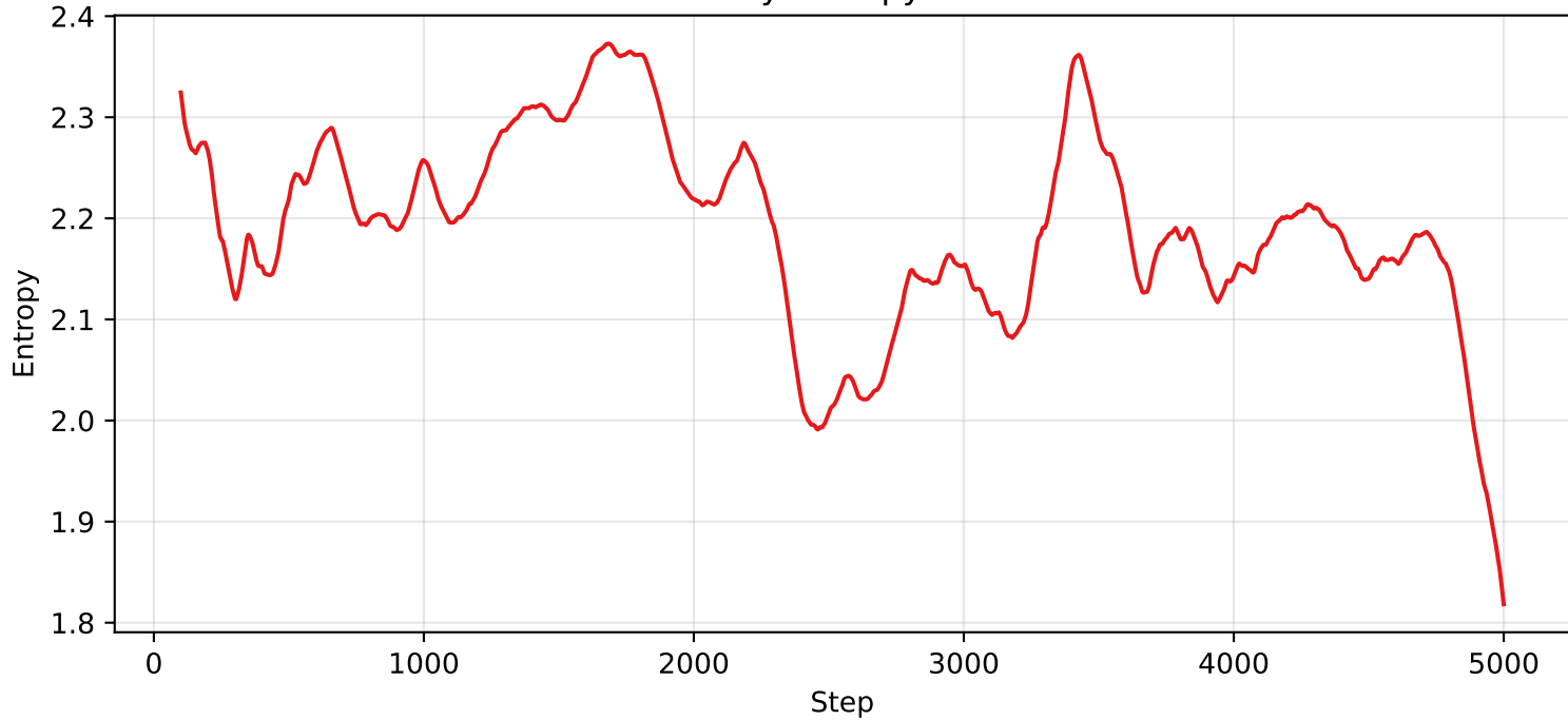
A2C - Policy Entropy Over Time
