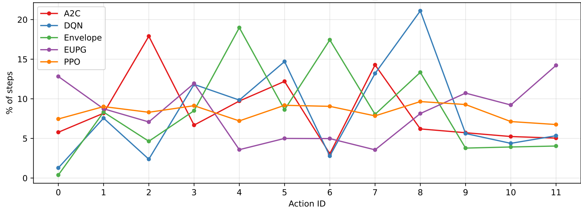
Action Selection Distribution Comparison (env_action, % of steps)
