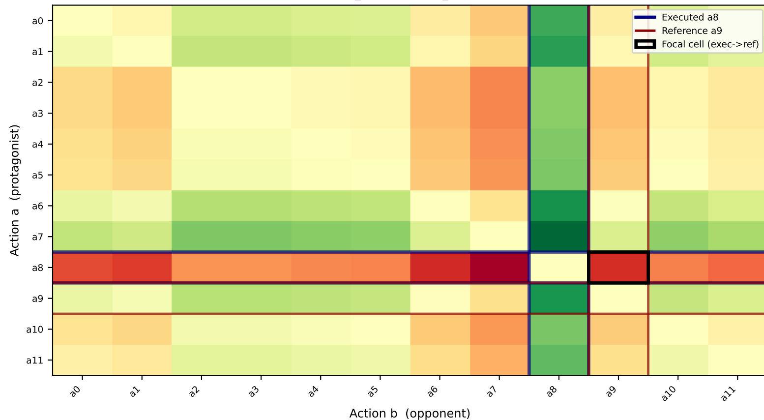
EUPG - Pairwise Q Advantage at Step 48 [Advantage] cell (a,b) = scalar_Q(a) - scalar_Q(b) >0: a is better
