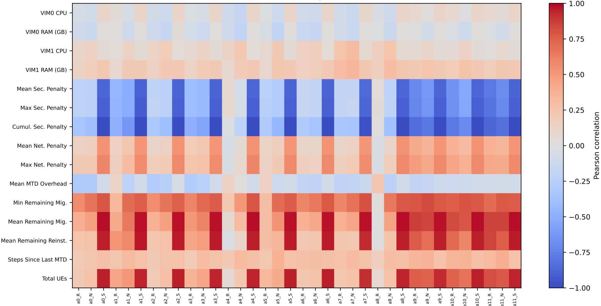
Envelope - Feature <-> Q-value Correlation (full log, 5,000 rows) Correlation between state features and per-action Q-value estimates
