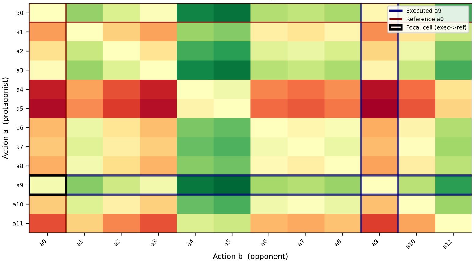
Envelope - Pairwise Q Advantage at Step 103 [Advantage] cell (a,b) = scalar_Q(a) - scalar_Q(b) >0: a is better
