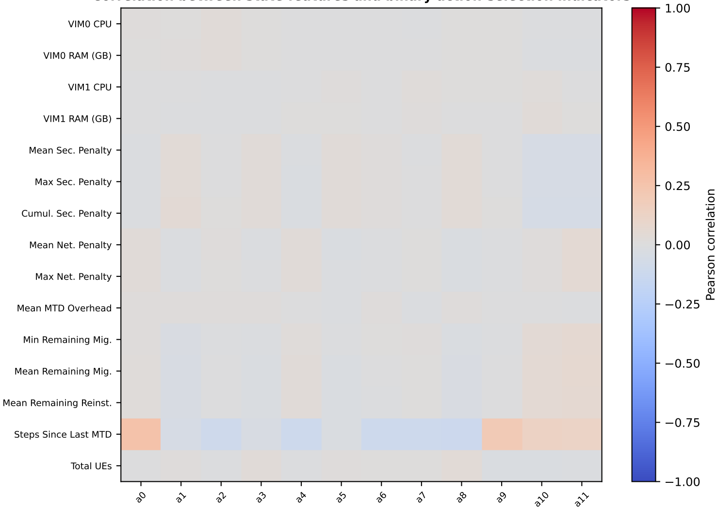
PPO - Feature <=> Action Selection (full log, 6,144 rows) Correlation between state features and binary action-selection indicators
