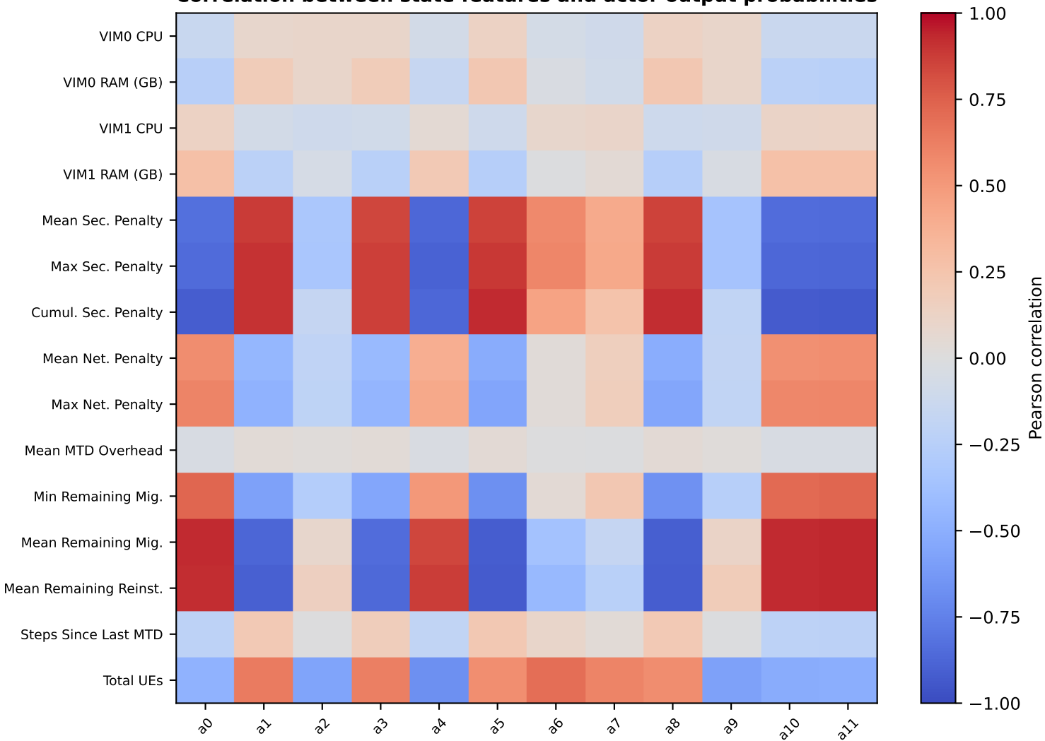
PPO - Feature <-> Policy Probability (full log, 6,144 rows) Correlation between state features and actor output probabilities
