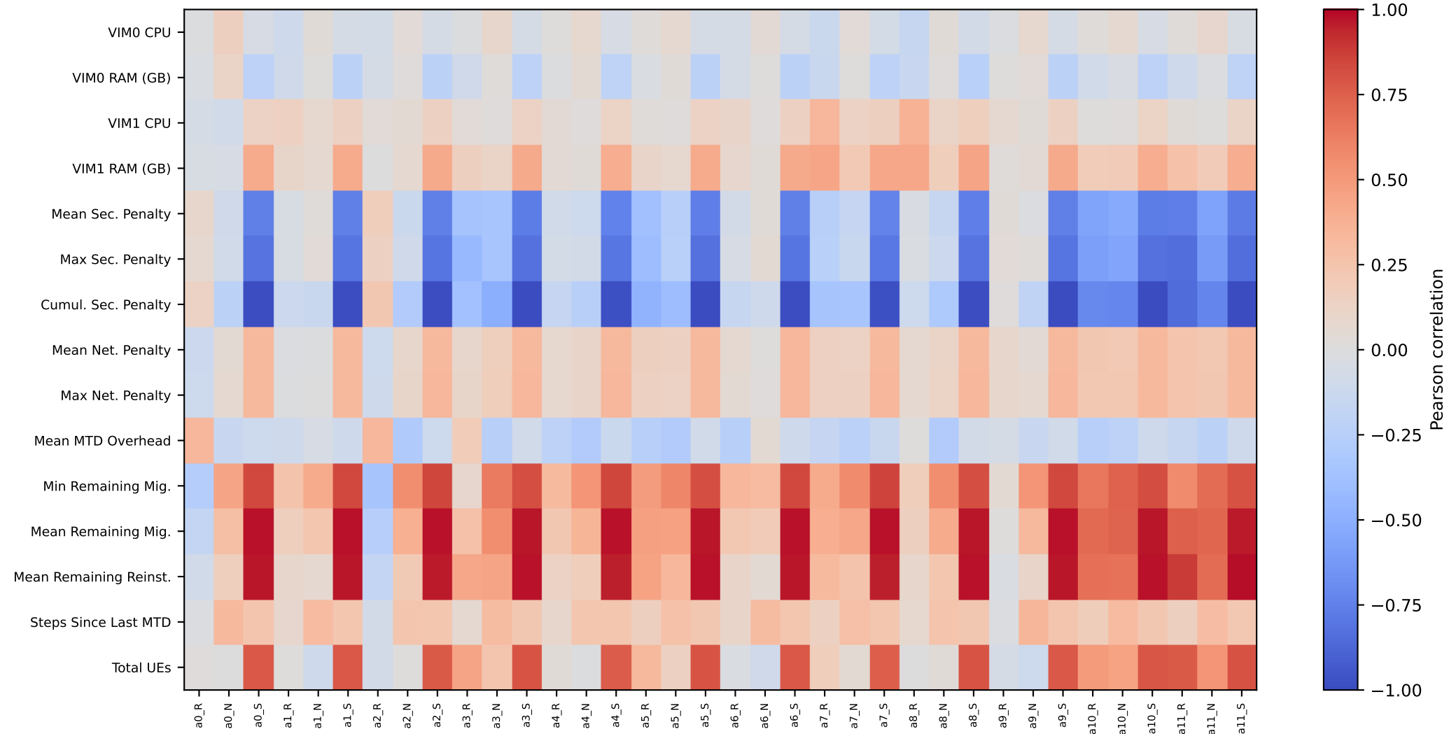
Envelope - Feature ↔ Q-value Correlation (full log, 5,000 rows)
