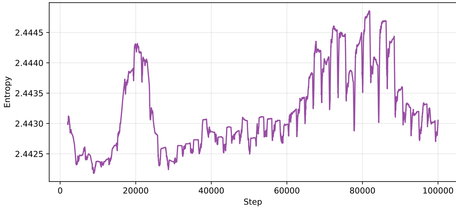
EUPG - Policy Entropy Over Time
