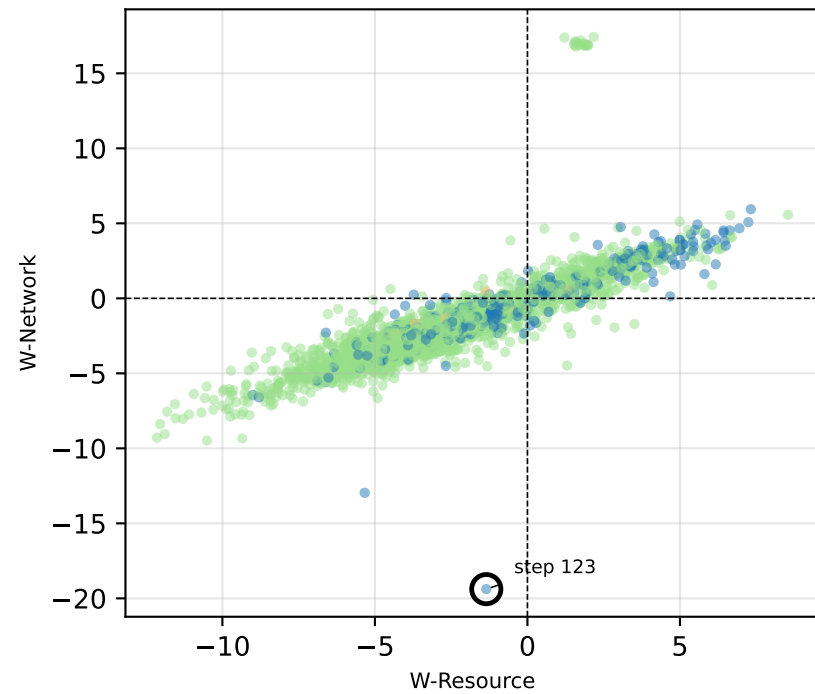
Advantage (match=True)
