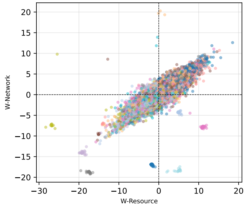
Regret (match=False)
