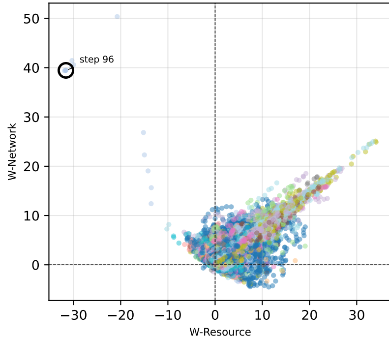
Advantage (match=True)
