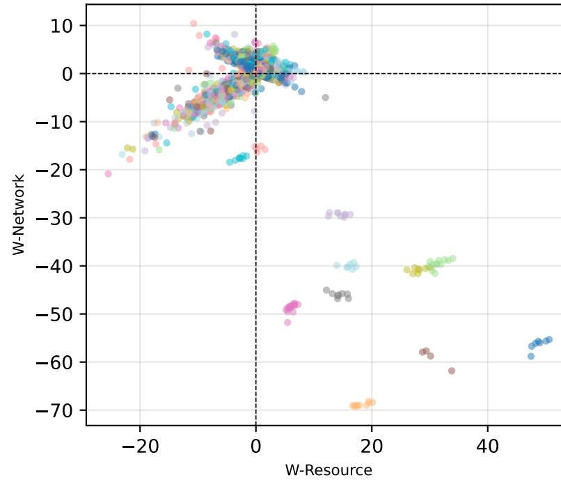
Regret (match=False)
