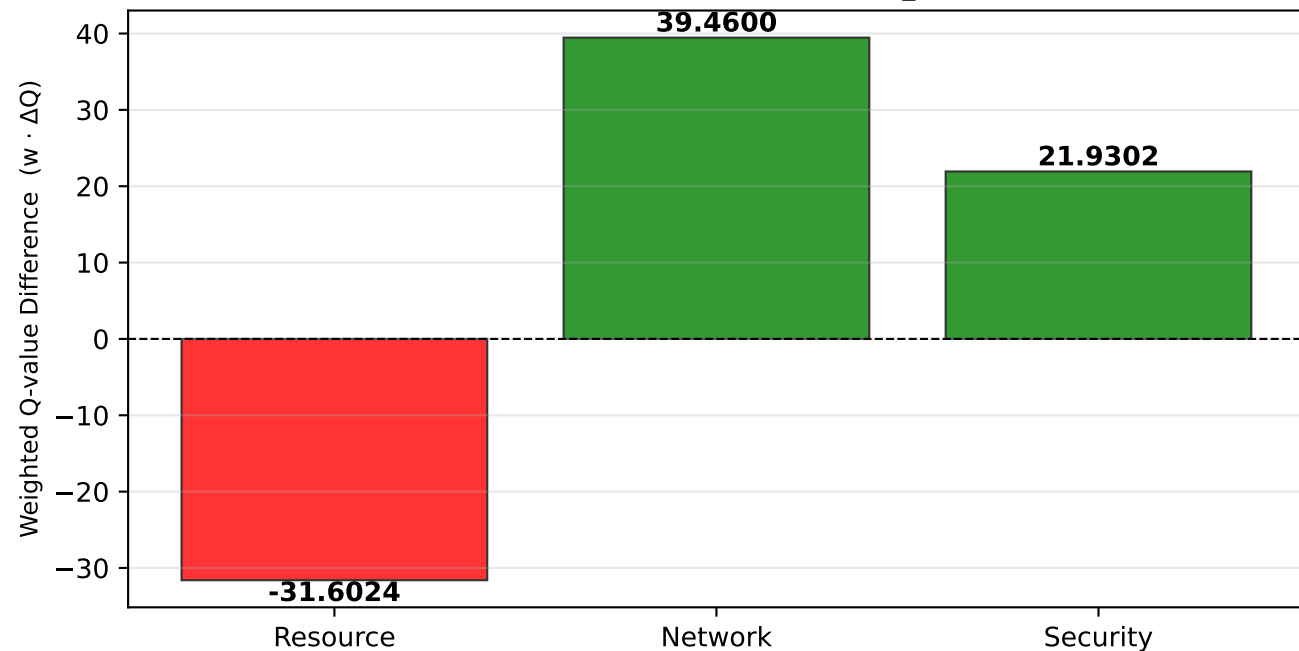
Envelope - Single-Step RDX at Step 96 [Advantage (env==ref) ✓] Best Action 1 vs Alt Action 3 (env_action=1)
