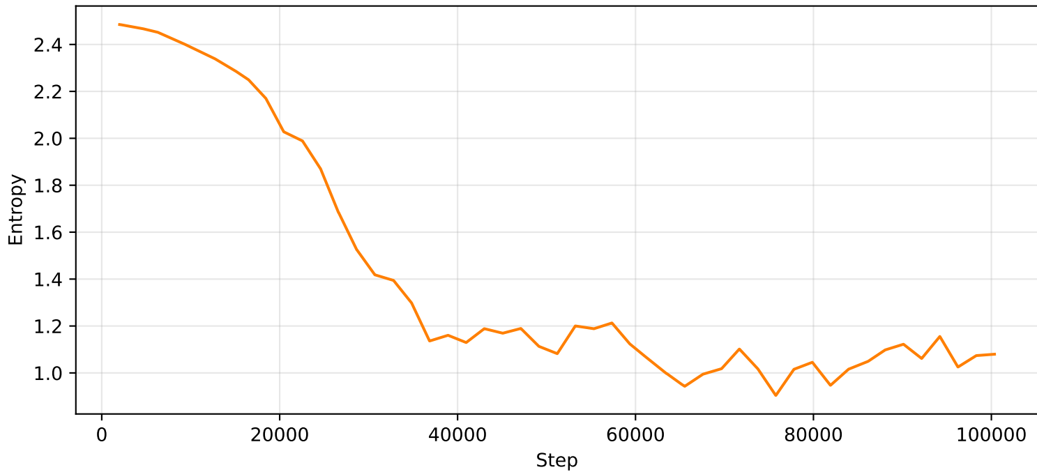
PPO - Policy Entropy Over Time
