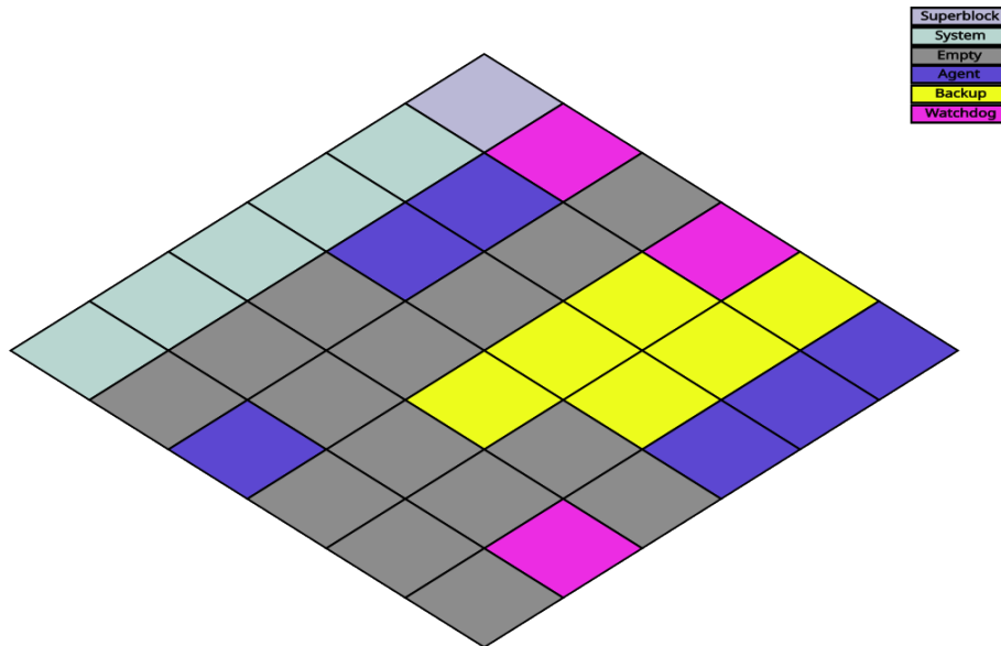
Figure 4: Statemap showing the actual state of the system.
