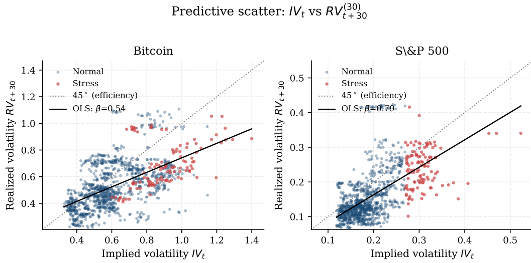
Figure 4.2. Predictive scatter of RV_{t+30}^{(30)} against IV_t for Bitcoin (left) and the S&P 500 (right). The dotted grey line is the 45° efficient frontier; the solid black line is the OLS fit on the full sample. Red dots mark days flagged as stress in each market.
