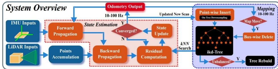
Figure 2: FAST-LIO2 front-end architecture, reprinted from Xu et al. [1]. In this project, object information from MCTrack is injected into the point-cloud preprocessing pipeline to realize adaptive down-weighting of dynamic points.
